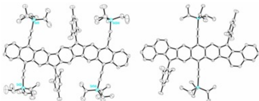
Figure. X-ray crystal structures of two \pi -expanded molecules recently prepared by the Haley group.
